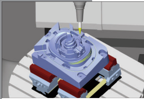
Virtual Machining in CAM: M+M's hyperMILL
